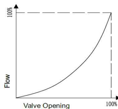
Opening flow characteristics
